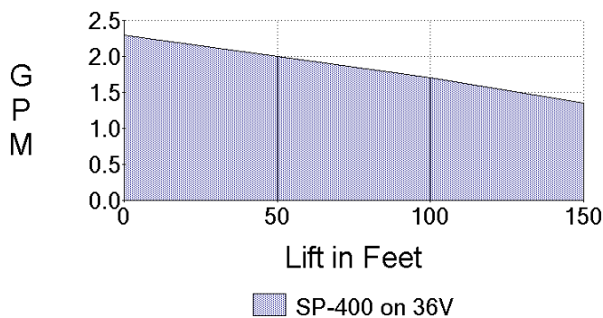
Pump Curve
